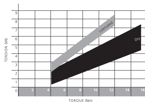
Fastener Lubrication
